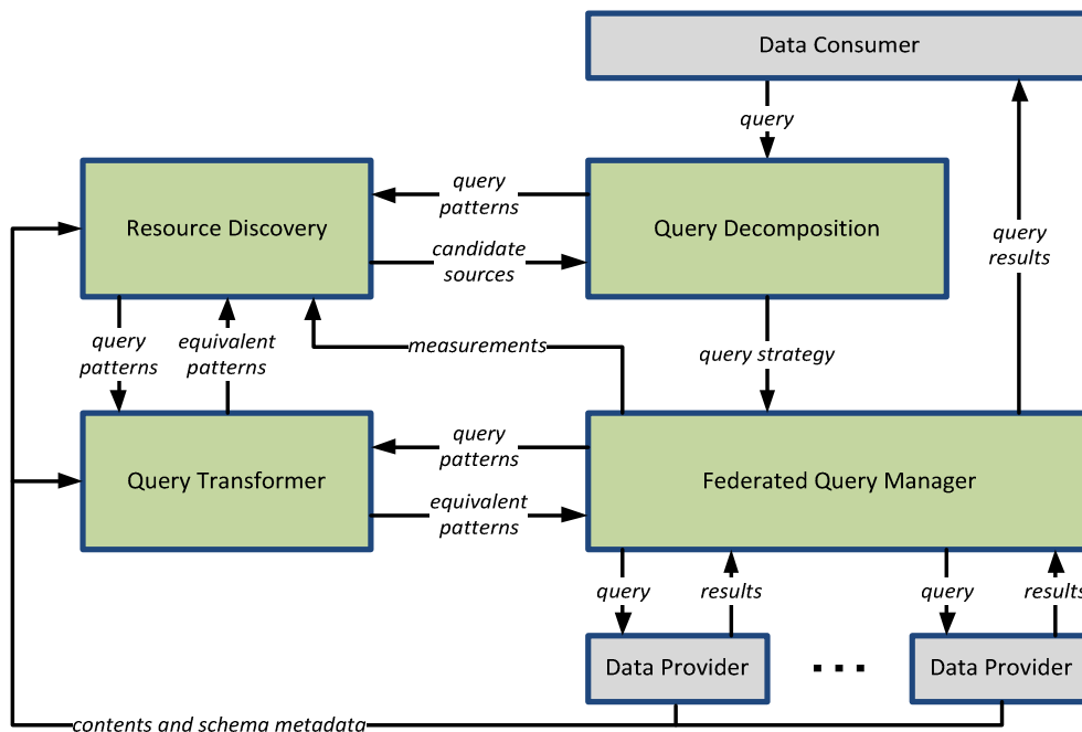
Figure 1: The architecture of the SemaGrow Stack.
